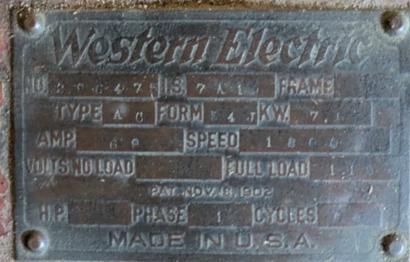
Nameplate for Item 6
